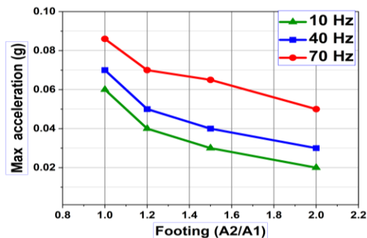
Fig. 17 Relation of maximum acceleration and area ratios footings
